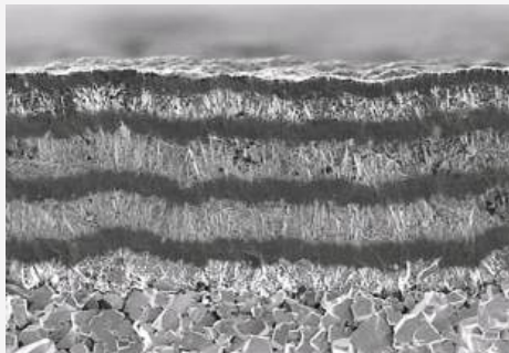
Multilayer Diamond Coating
